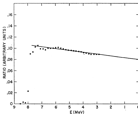
FIG. 5. The ratio of the cumulative gamma-ray spectra, as observed in 3 in. \times 3 in. NaI, from resonance and thermal capture. A straight line is fitted to the data between 3 and 7 MeV, and used to extrapolate the ratio to zero energy.
